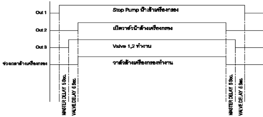
Timing Diagram
